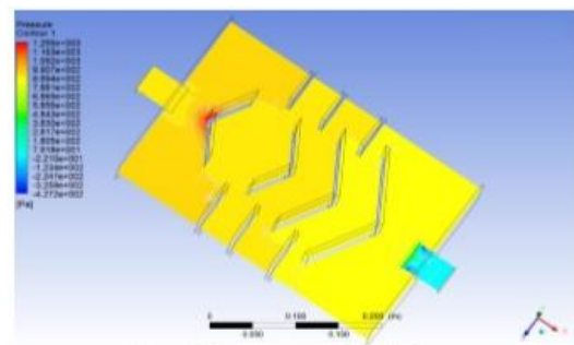
Figure 4- 3 Design 2's pressure curve is being studied.
