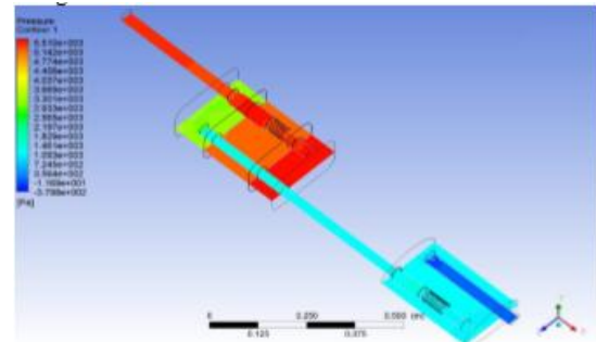
Figure 4- 7 In Design 6, the pressure curve is depicted.
