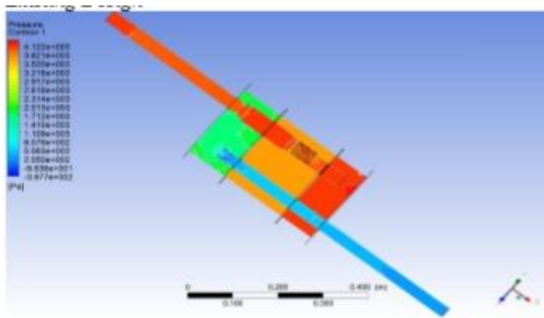
Figure 4- 1 A pressure contour is formed by the current.
