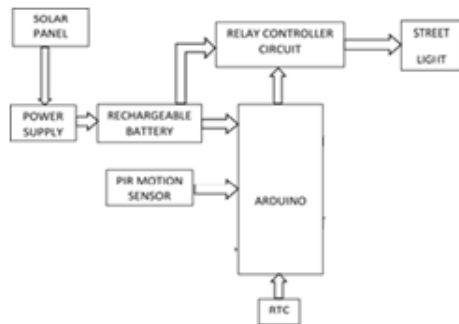
Fig-2: Block Diagram of All-in-One Solar Street Light
